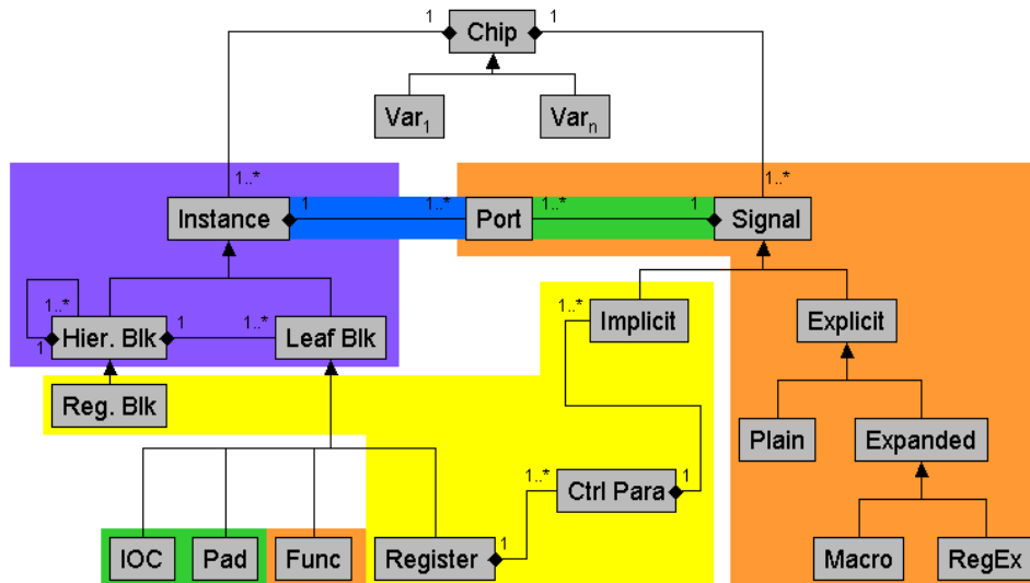
Figure 8: Data Model
