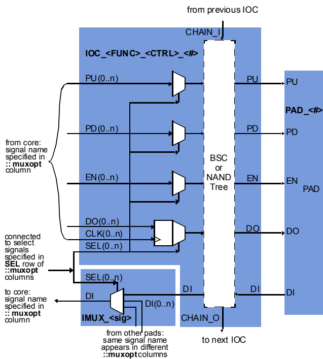
Figure 5: IO Control Cell
